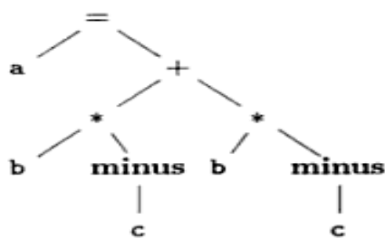
(a) Syntax tree
