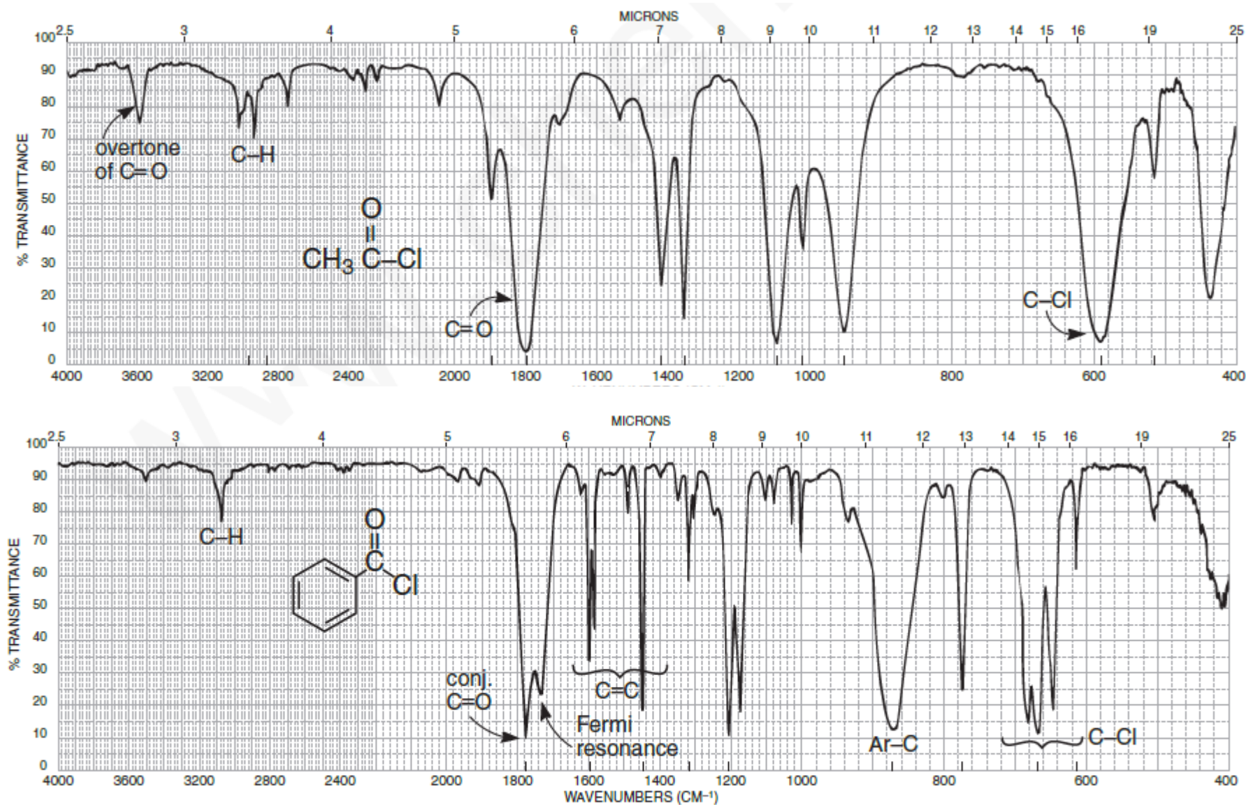
The infrared spectrum of benzoyl chloride (neat liquid, KBr plates).
