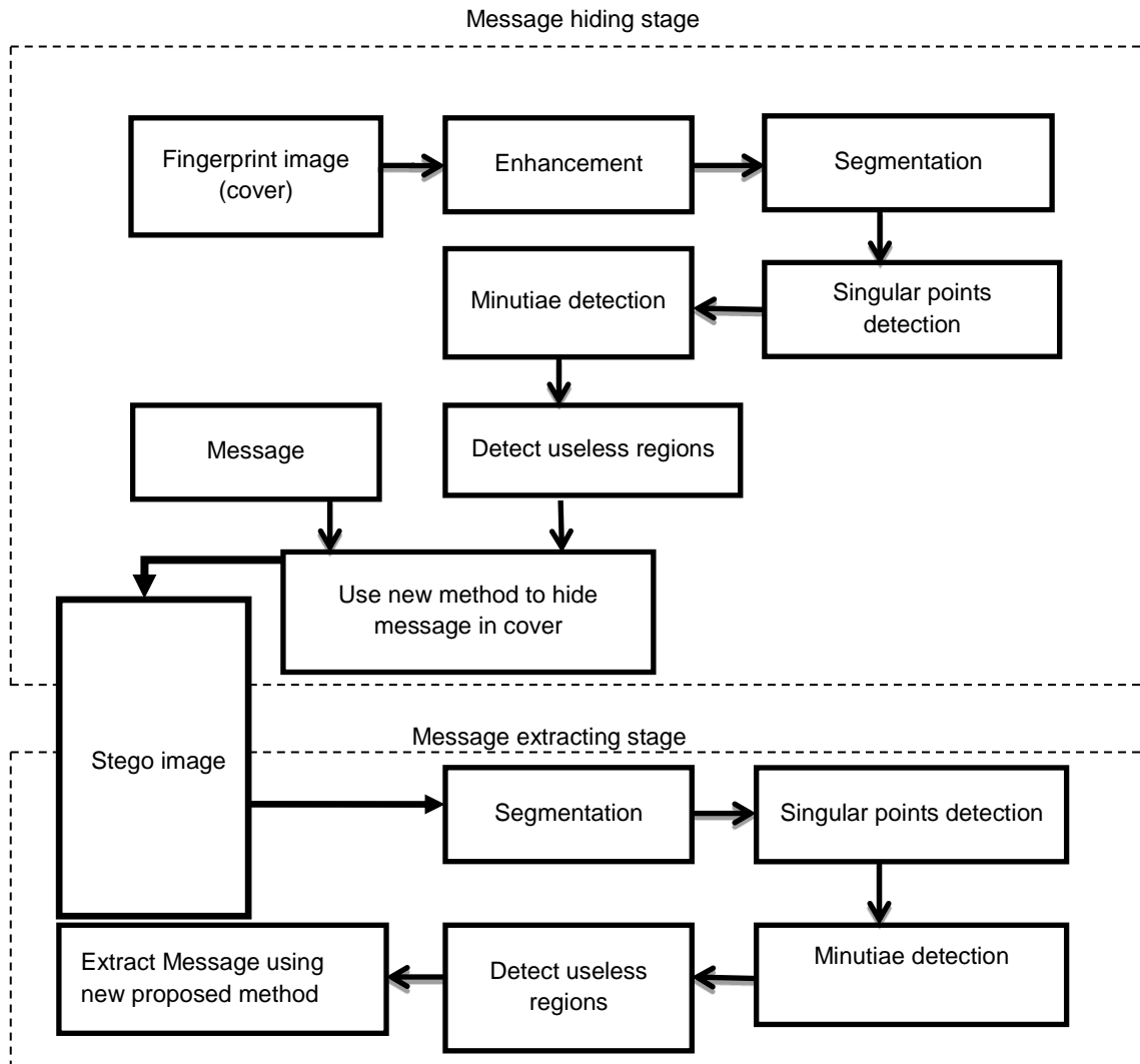
Figure (5) block diagram of proposed system
