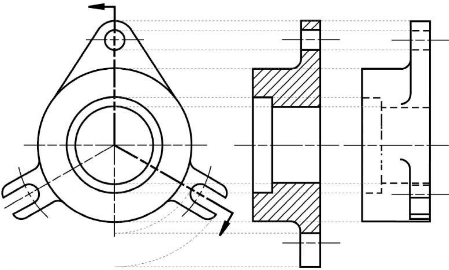
Aligned section using the conventions of revolution.
